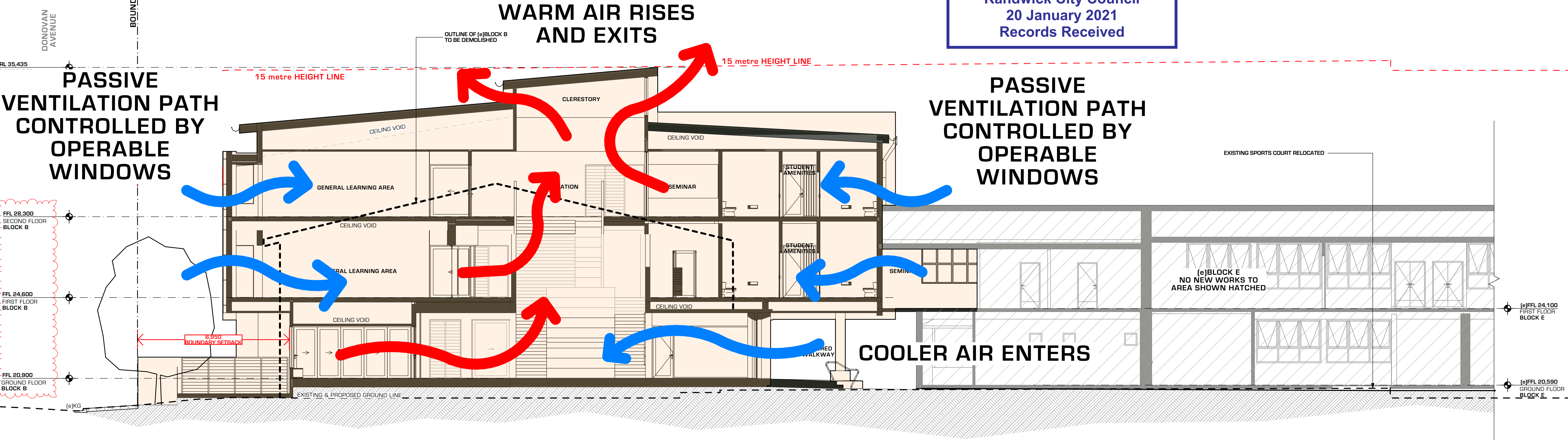
S.01 SECTION 01 - BLOCK B
